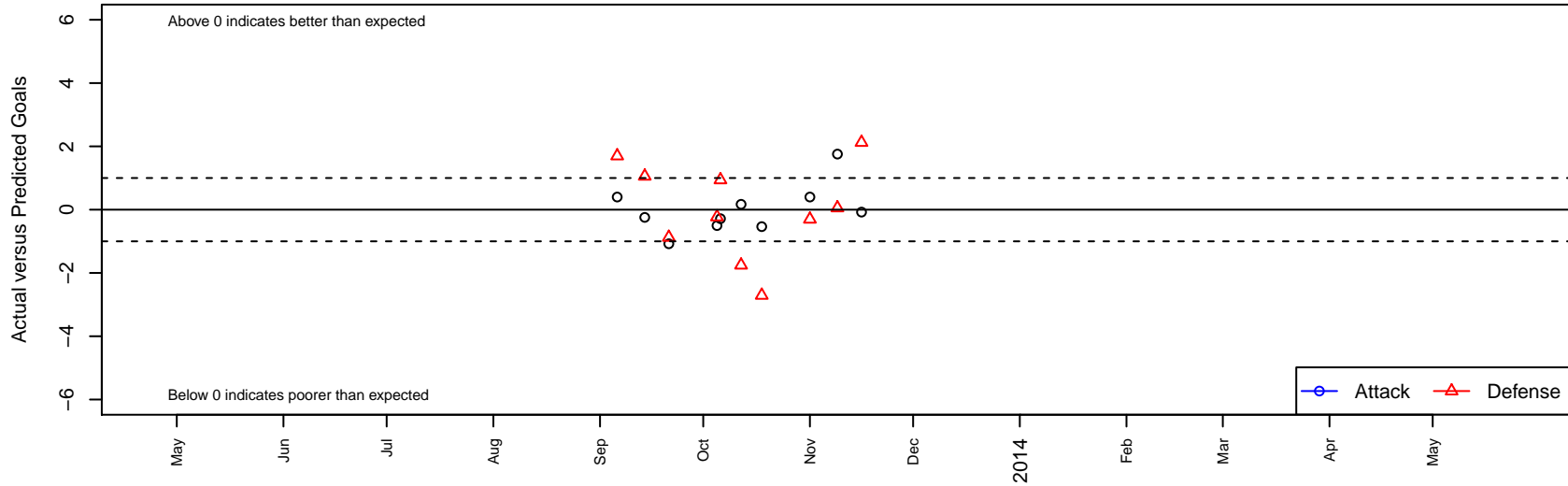
Sacramento United Extreme Red G02 Dots are actual minus expected GF (blue circles) and GA (red triangles). Blue line is smoothed change in attack strength. Red is smoothed change in defense strength.
